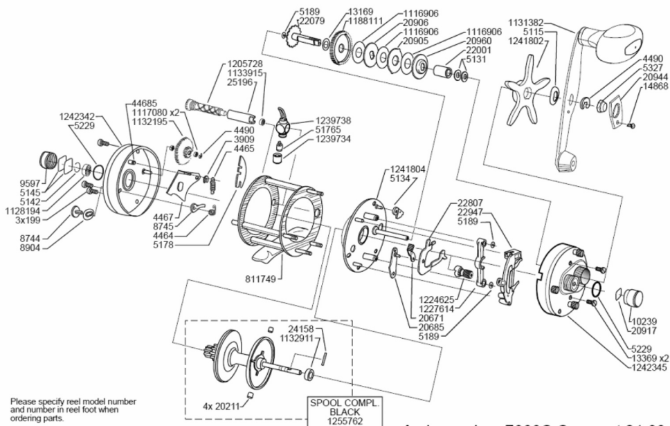
Ambassadeur 7000C Compact 21 00
